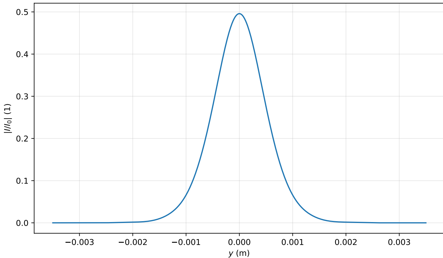
Intensity profile I(x=0, y, z=3.901)/I_0 , P_{in}=0.6P_{cr} , artificial time
